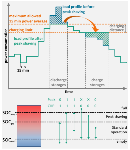
Schematic representation of the algorithm for peak shaving (top) and peak shaving by CHP (bottom)
